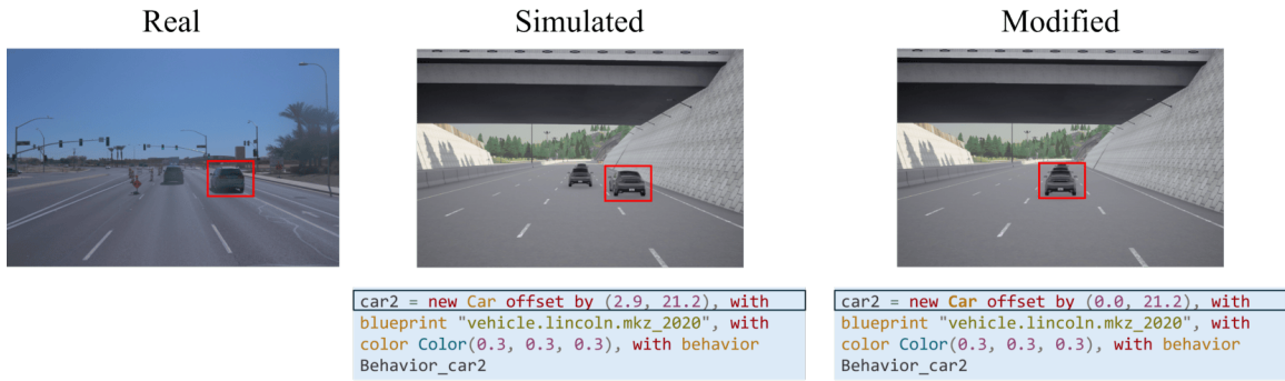
Figure 10: We can manipulate the initial position of the vehicle. The position is defined as a pair of coordinates relative to the ego vehicle frame. The x -coordinate has been shifted to 0.0, which causes the vehicle to be translated to the left lane. This shows a way to generate a new scenario to allow an autonomous driving model to handle diverse situations. The relevant modified vehicle is indicated in the illustration.
